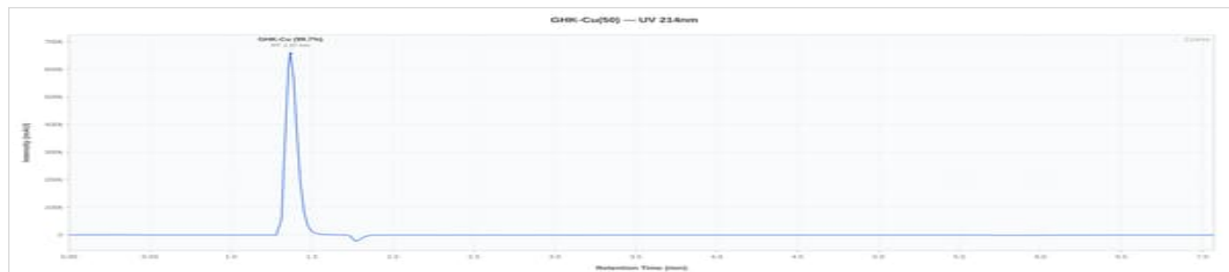
GHKcu 50mg - KYB-26CU50:01: UV Chromatogram
